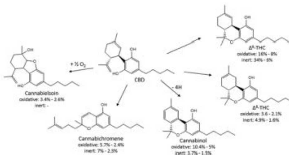
Figure 1. The major thermal decomposition routes of CBD in inert (helium) and oxidative (9% oxygen in nitrogen) atmosphere in a temperature range of 250–500 °C.
